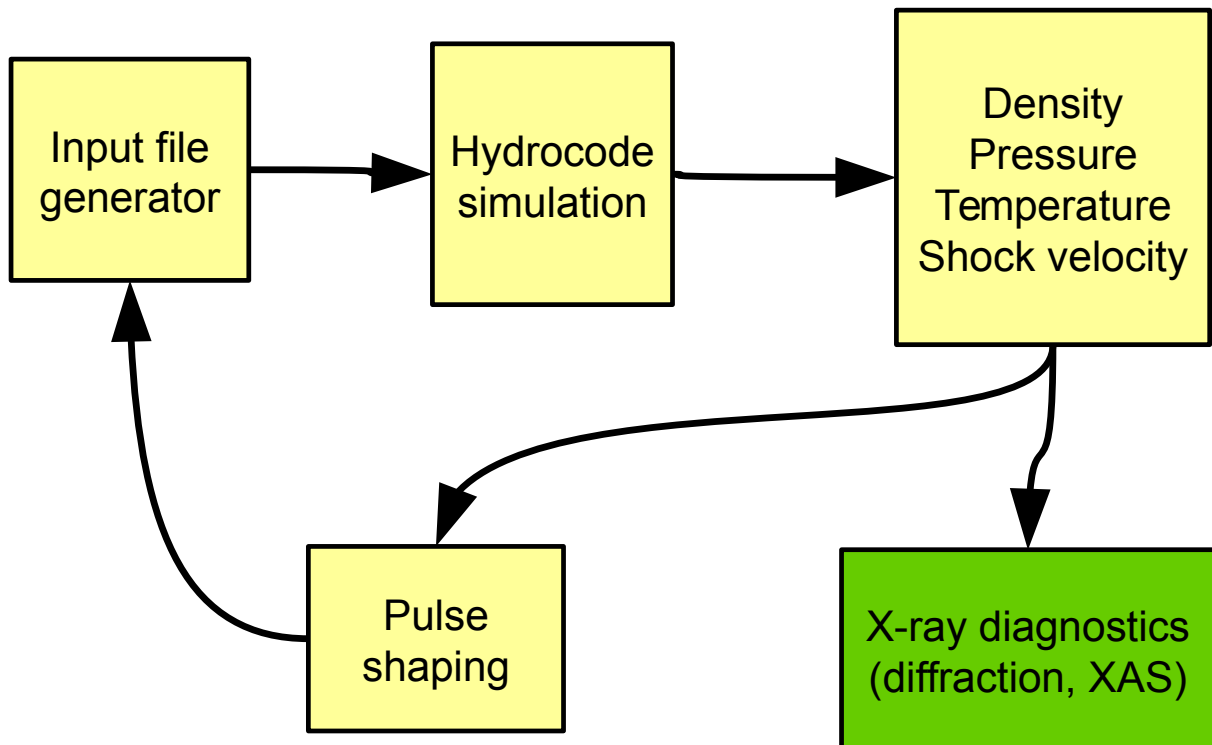
Figure 2: Optimization of pulse shapes for low isentropic compression. The output of radiation-hydrodynamics simulations is fed into a pulse shape generator to optimise the laser-matter interaction for maximum compression at low temperature increase. Once an optimized pulse is generated, the simulation continues with calculating the x-ray – matter interaction and synthesizing the diagnostic signals
